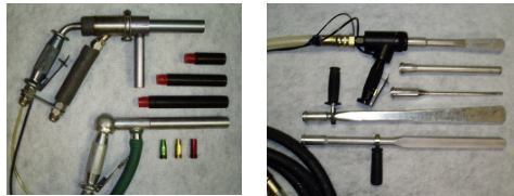
Assorted nozzles and guns, in high flow and low flow configurations, utilizing single hose—airlock, or dual hose—venturi design.
